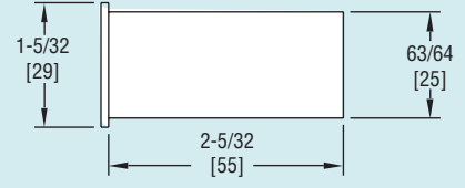
Panel Cutout 2.36" x 1" (60 x 26 mm)
